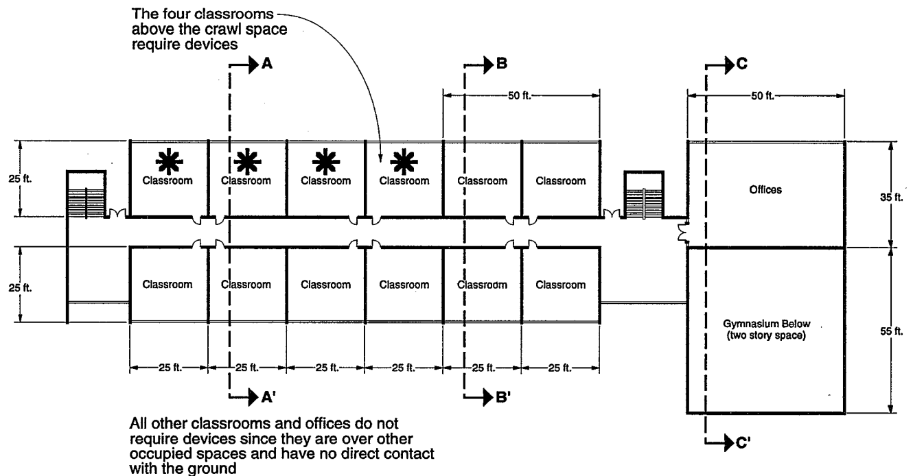
Correct answer for Figure 4-8: Upper level plan of a typical school showing placement of detectors.
