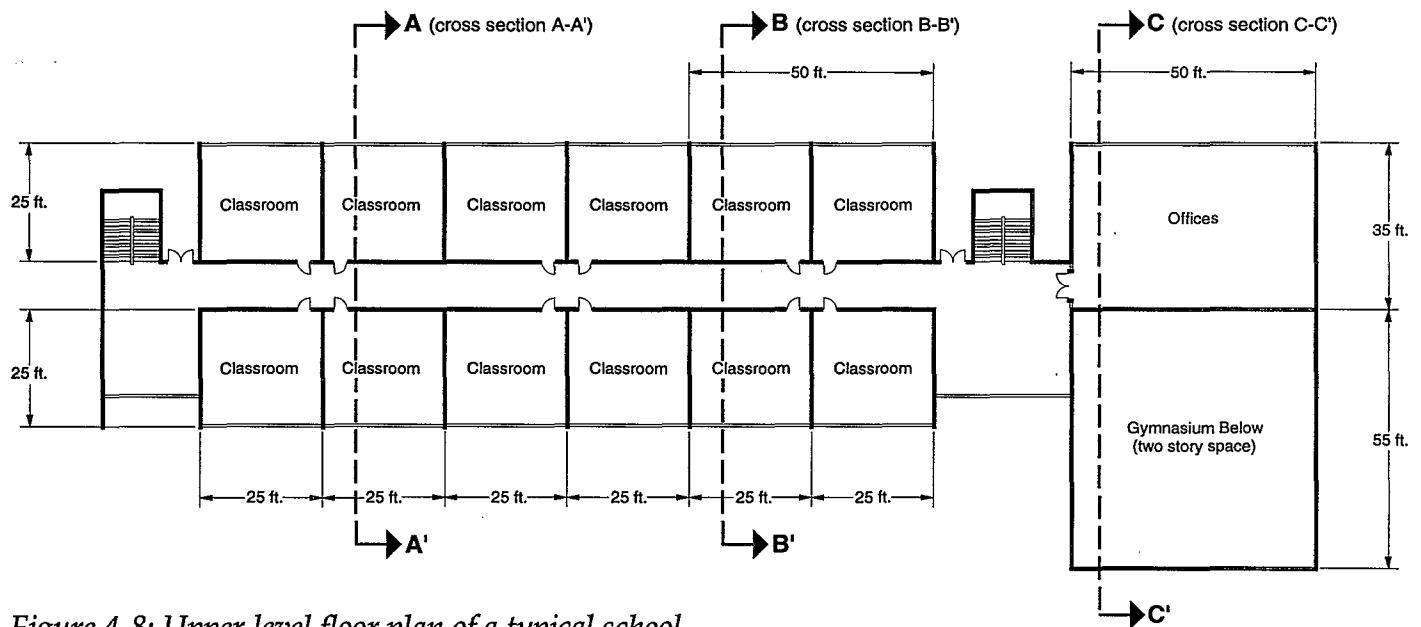
Figure 4-8: Upper level floor plan of a typical school.
