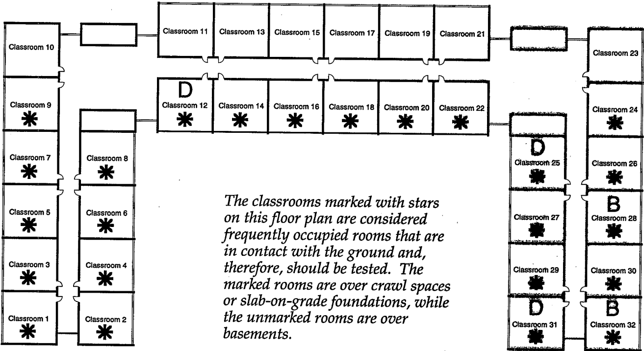
Correct answers for Activity 5-2: Duplicate device placement for floor plan of school.
