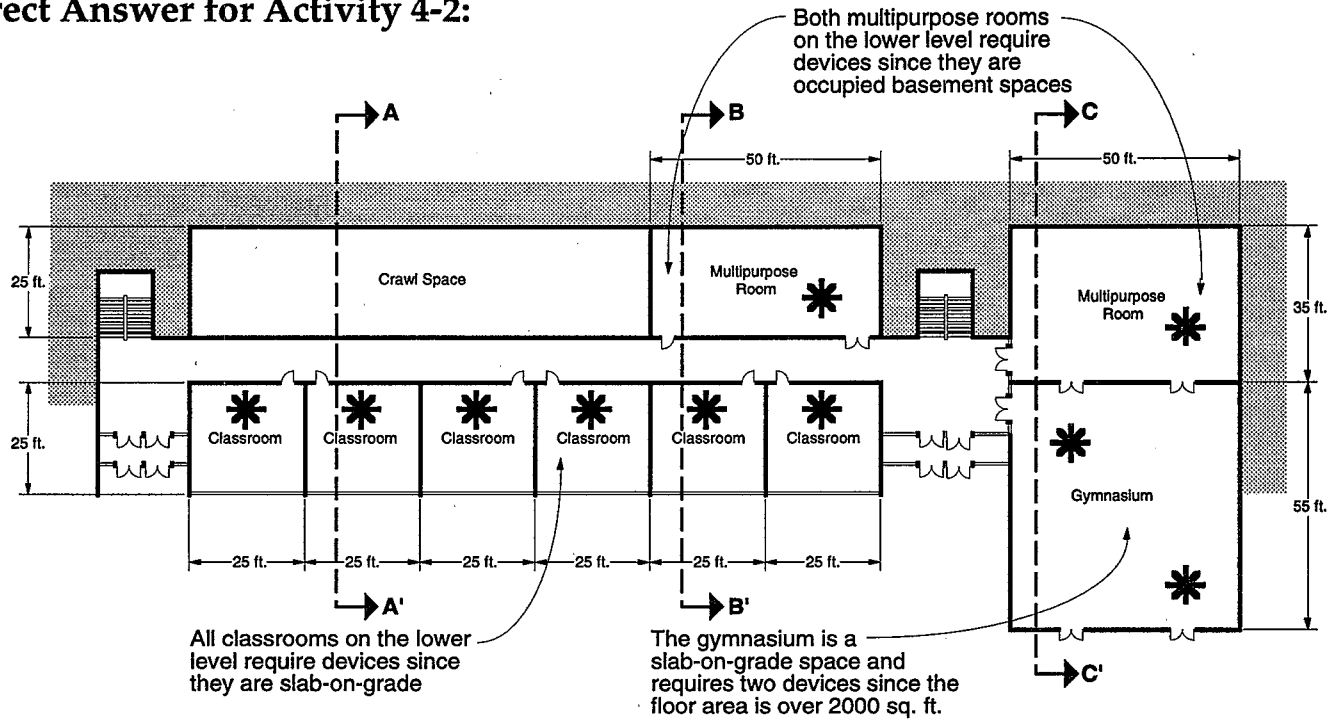
Correct answer for Figure 4-7: Lower level plan of a typical school showing placement of detectors.
