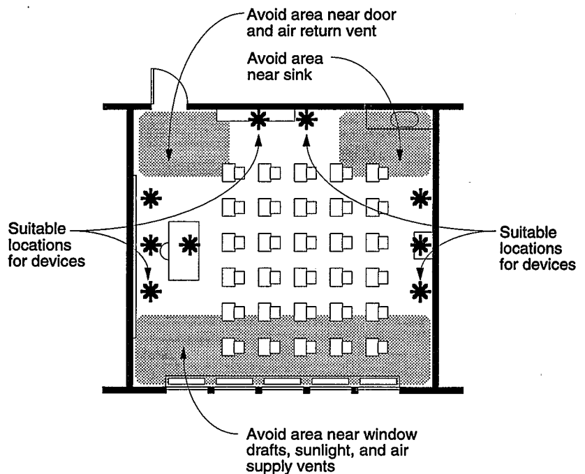
Figure 4-9: Plan of a typical classroom showing several suitable locations for placement of detectors. Only one detector is required for this room.
