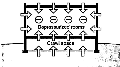
Figure 1-4: Some mechanical ventilation systems are not properly balanced resulting in depressurization of the interior spaces in a building. This can induce radon to enter spaces and must be addressed in a mitigation effort.
