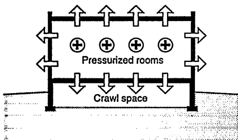
Figure 1-3: Mechanical ventilation can be designed to pressurize the interior spaces in a building by bringing in outdoor air. This may help reduce radon entry by pressurizing the building and diluting radon.
